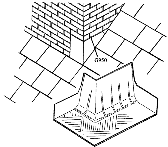
4) GW293CC LH CORNER CATCHMENT TRAY
